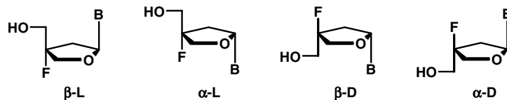
2',3'-Dideoxy-3'-fluoroapiofuranosyl nucleosides
